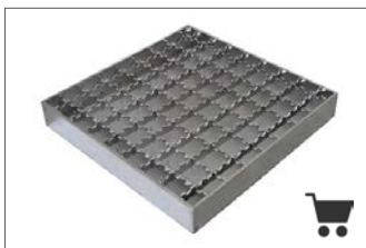
Maasrooster 25 x 25 x 2 mm Belasting 15 kN licht transport
